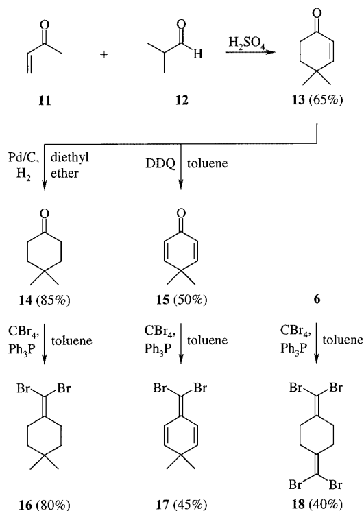
Scheme 3. Preparation of starting materials for cross-conjugated enynes
