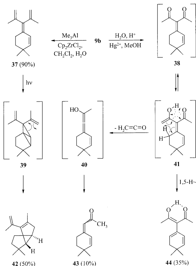
Scheme 8. The chemical behavior of 9b
