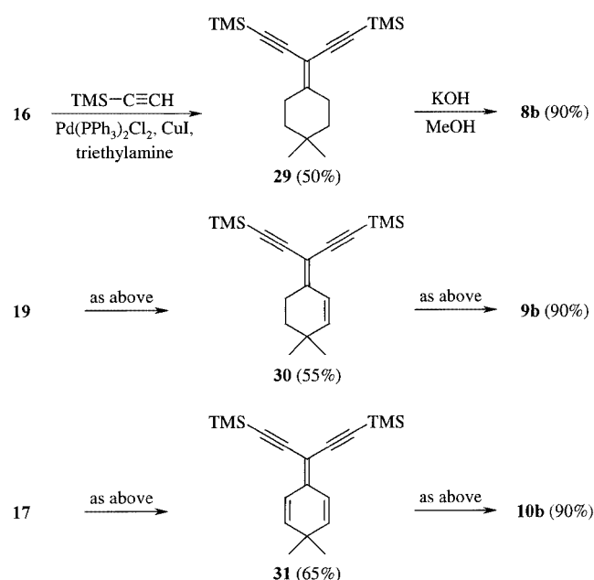
Scheme 6. Preparation of the parent systems 8b–10b
