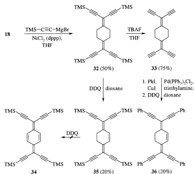
Scheme 7. En route to tetraethynyl- p -quinodimethane derivatives
