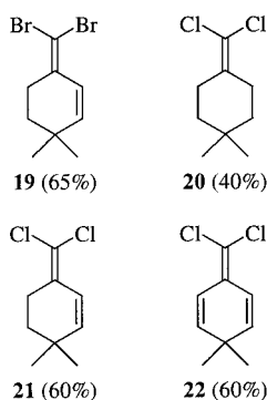
Scheme 4. Additional dihalo olefins
