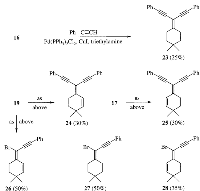
Scheme 5. Preparation of phenyl-substituted cross-conjugated enynes
