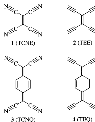
Scheme 1. A selection of important cross-conjugated systems
