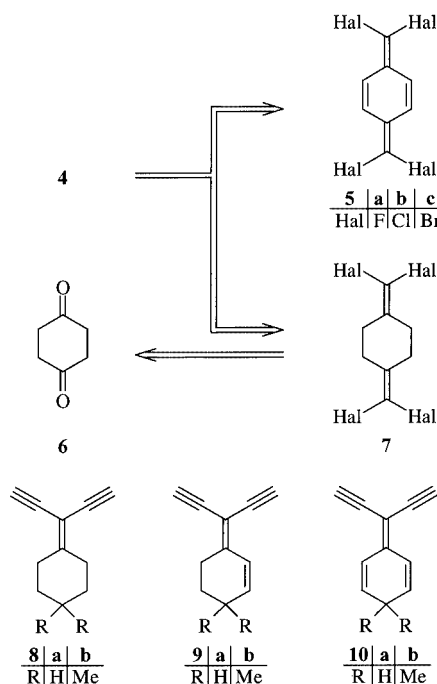
Scheme 2. Retrosynthesis of tetraethynyl- p -quinodimethane
