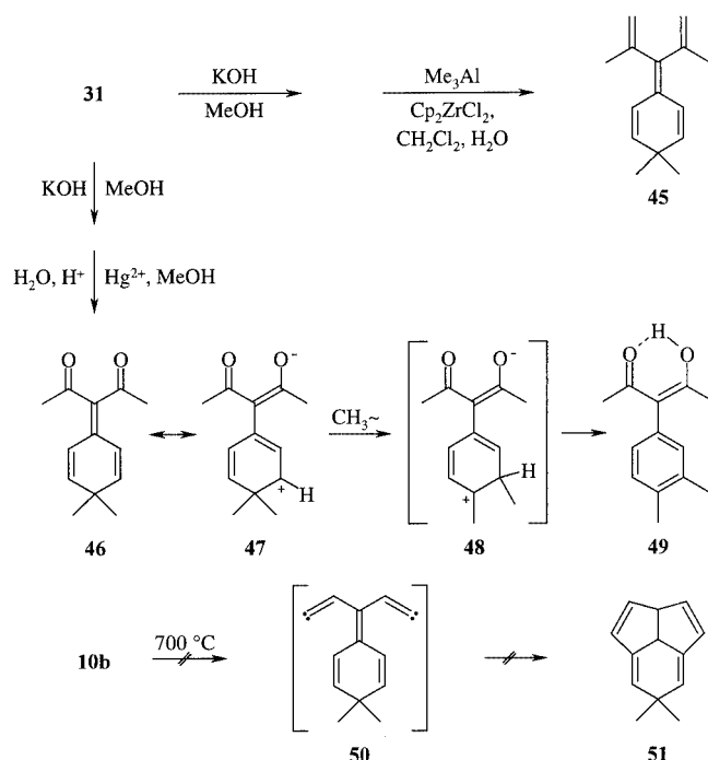
Scheme 9. The chemical behavior of 31
