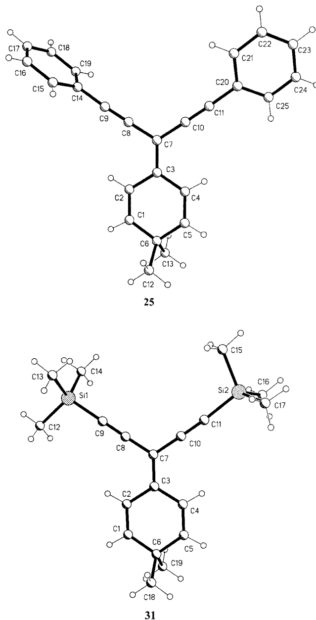
Figure 1. The structures of 25 and 31 in the crystal
